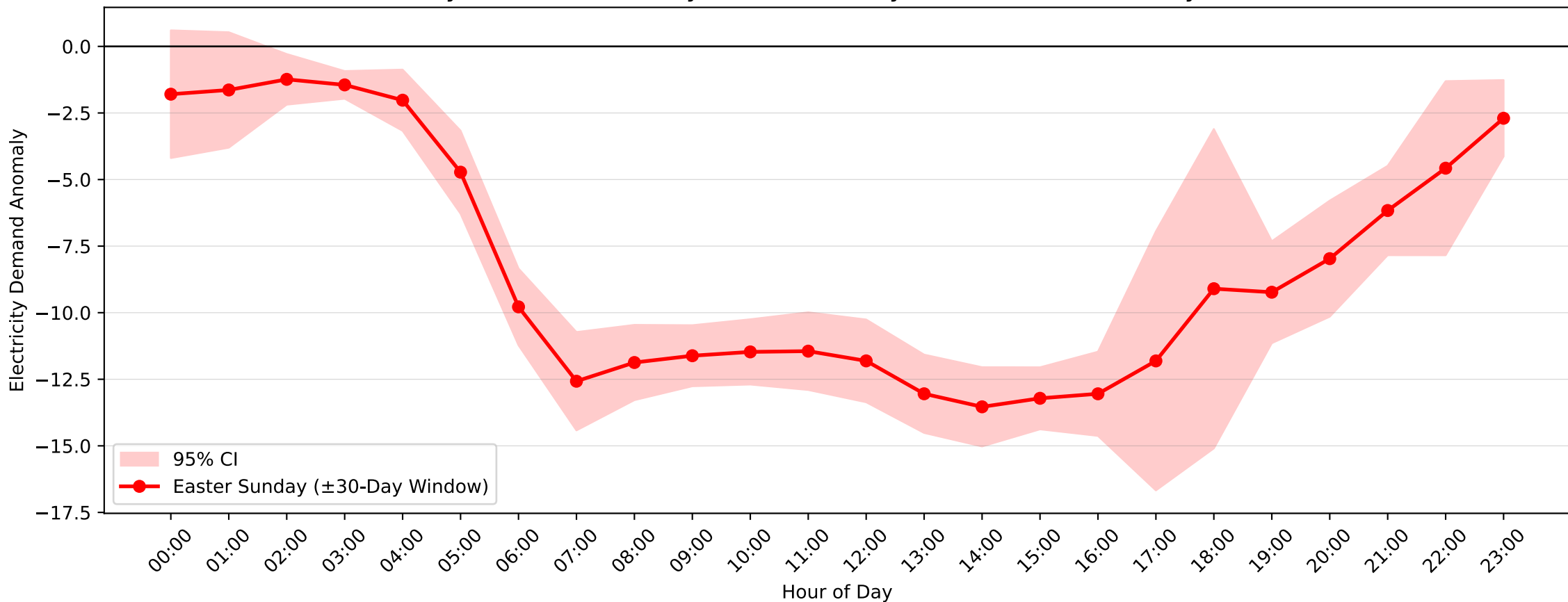
Hornsby Demand Anomaly: Easter Sunday (2008-2009, \pm 30 -Day Window)
