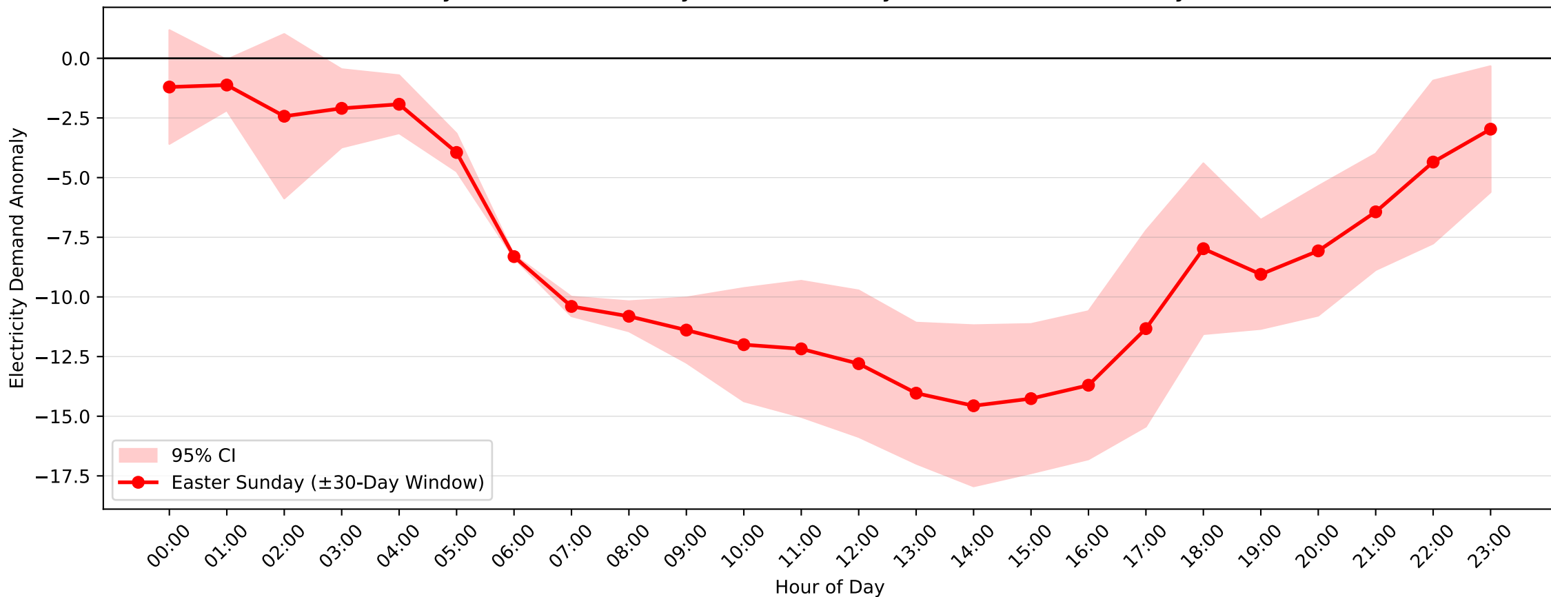
Hornsby Demand Anomaly: Easter Sunday (2009-2010, \pm 30 -Day Window)
